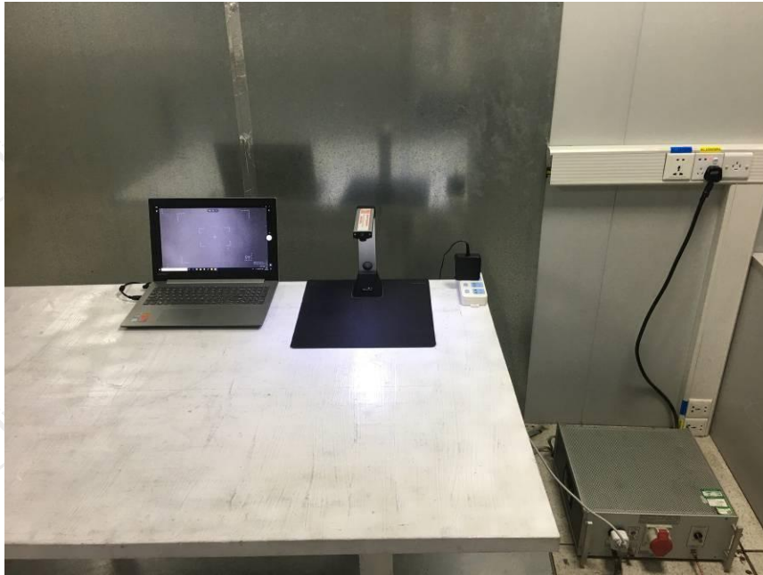
Conducted Emission Test View
